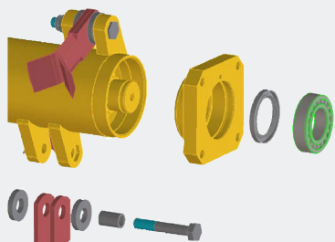
2300 RPM high speed rotor with fully inclosed bearings
