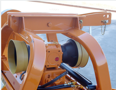
Heavy duty gearbox mount
