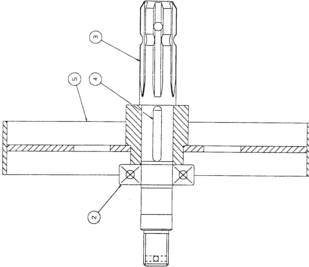
ASSEMBLY: -7703545 PTO SHAFT & PULLEY
