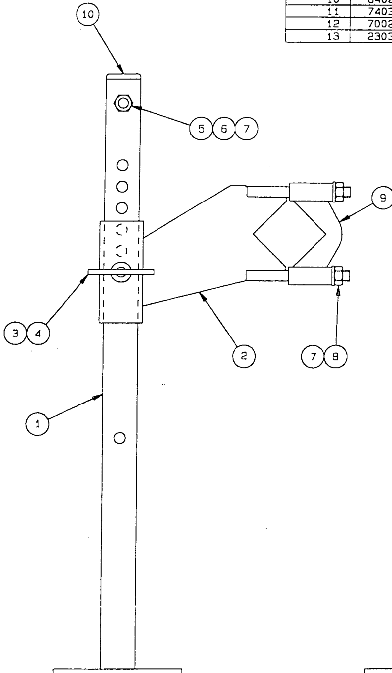
ASSEMBLY: -7702095 (ITEMS 1-10)
